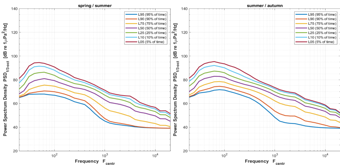
Fig. 4.3.2. Mean values of the power spectrum density of the underwater noise in the 1/3-octave frequency bands PSD [dB re 1 \mu\text{Pa}^2\cdot\text{Hz}^{-1} ]. As per measurements data obtained during the period between 2 May 2022 to 11 August 2022 (on the left) and between 12 August 2022 to 14 November 2022 (on the right).
