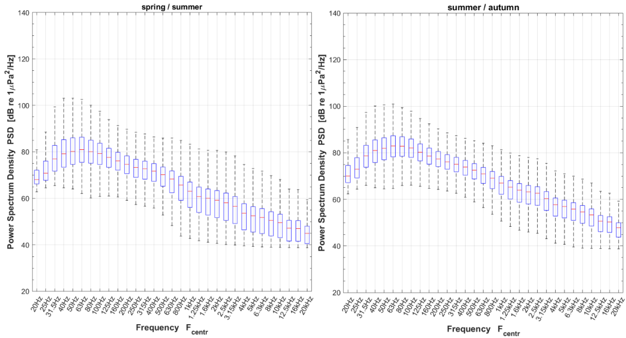
Fig. 4.3.1. Statistical distribution of the averaged power spectral density PSD [dB re 1 \mu\text{Pa}^2\cdot\text{Hz}^{-1} ] values of the underwater noise in 1/3-octave frequency bands. As per measurements data obtained during the period between 2 May 2022 to 11 August 2022 (on the left) and between 12 August 2022 to 14 November 2022 (on the right).
