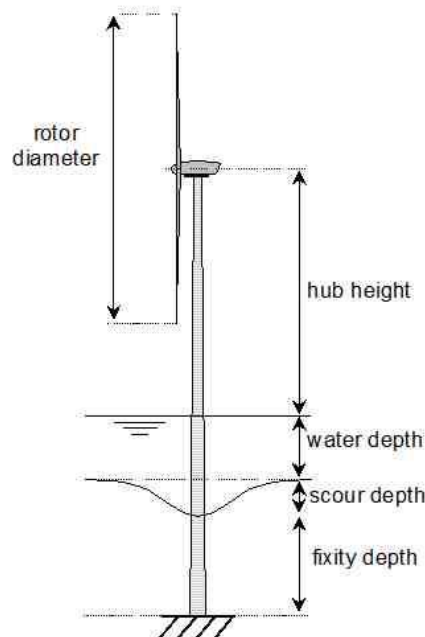
Fig. 1.1.2. WT height scheme (data by David Cerda Salzmänn, Delft University of Technology).
