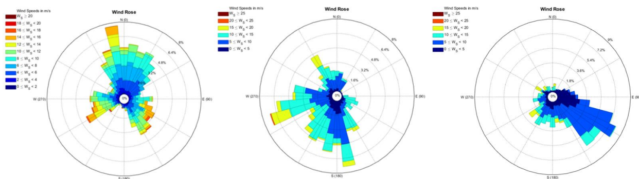
Fig. 4.2.3. The wind roses in summer (on the left), autumn (in the center) and in December (on the right) (based on 2022 Eolos data at E06 observation station).
