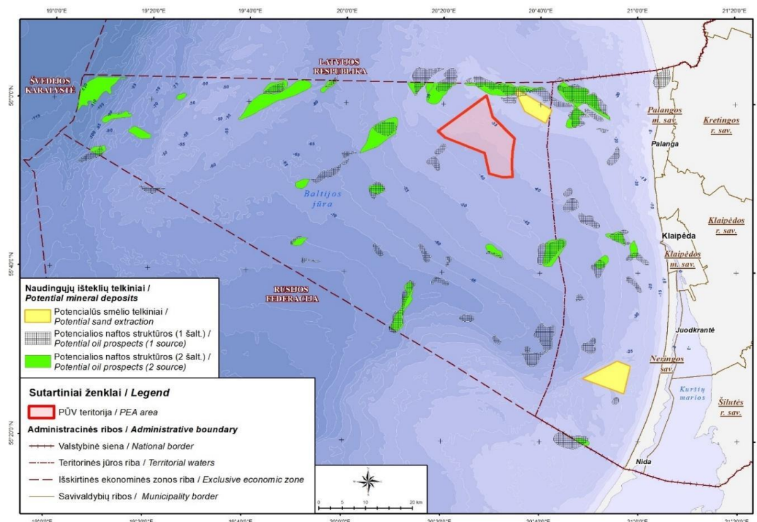
Fig. 4.4.7. Layout of the PEA area in respect of mineral deposits. Legend: source 1 - Underground Register, Lithuanian Geological Survey, Deposits of underground resources (with borders); source 2 – as per Fig. 4.4.4.
