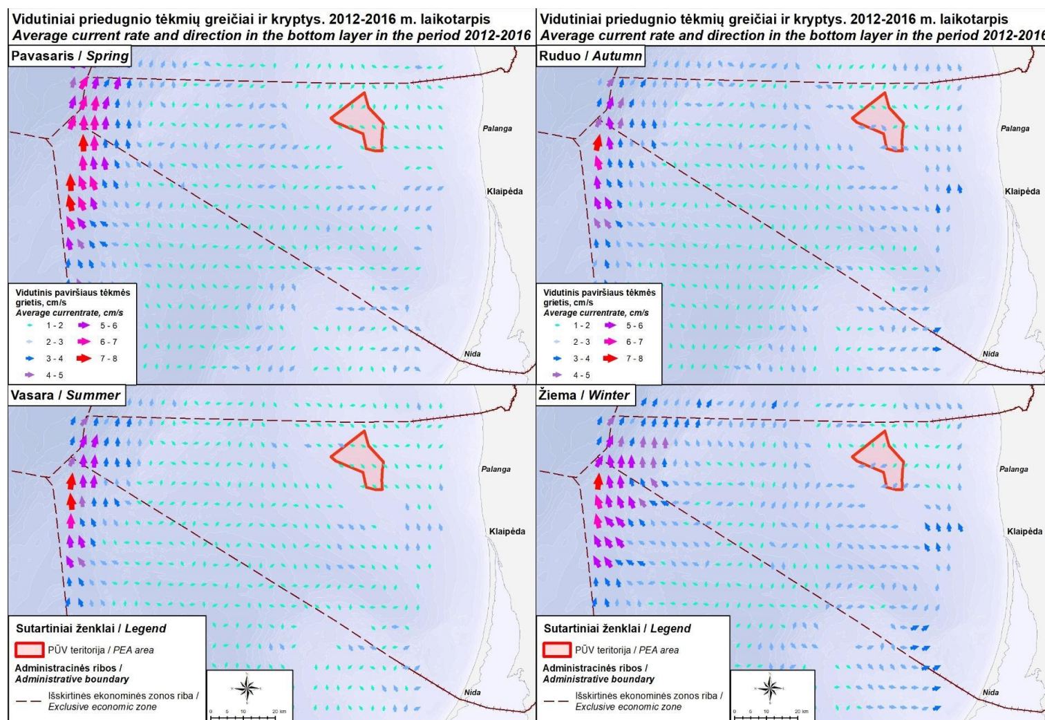
Fig. 4.1.5. Average current rate and direction in the bottom layer (as per data of 2012–2016, SMHI, Sweden).
